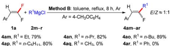
Scheme 5. Primary Alkylation of gem -Difluoroalkene under Transition-Metal-Free Conditions a,b
