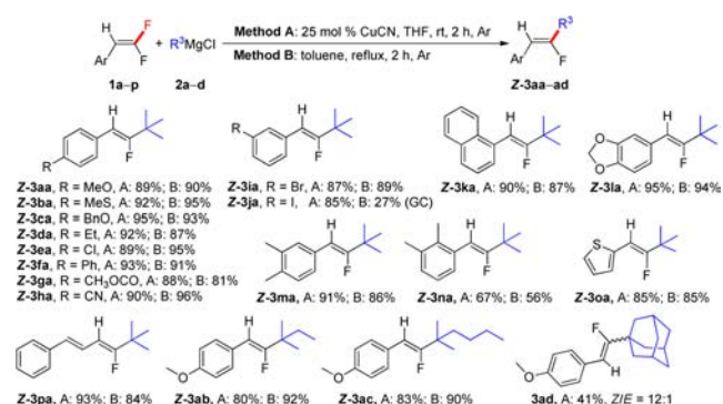
Scheme 2. Tertiary Alkylation of Various gem -Difluoroalkenes a,b
