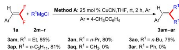
Scheme 4. Cu-Catalyzed Primary Alkylation of gem -Difluoroalkene a,b
