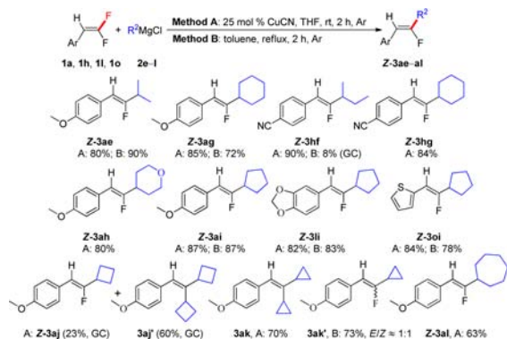
Scheme 3. Secondary Alkylation of gem -Difluoroalkenes a,b
