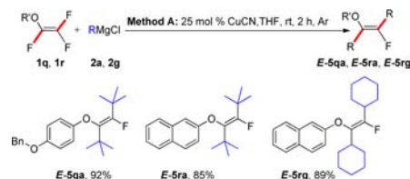
Scheme 6. Cu-Catalyzed Alkylation of ((1,2,2-Trifluorovinyl)oxy)arenes a,b
