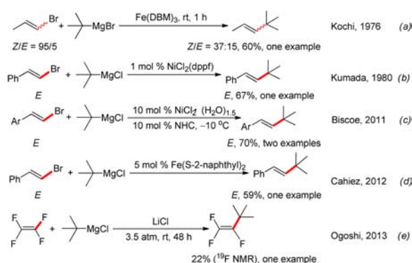
Scheme 1. Tertiary Alkylation of Alkenyl Halides
