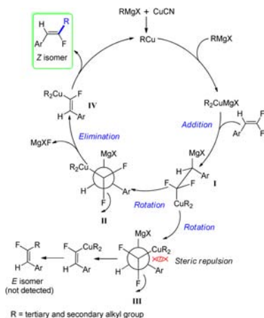
Scheme 7. Plausible Mechanism of Cu-Catalyzed Tertiary and Secondary Alkylation of gem -Difluoroalkenes
